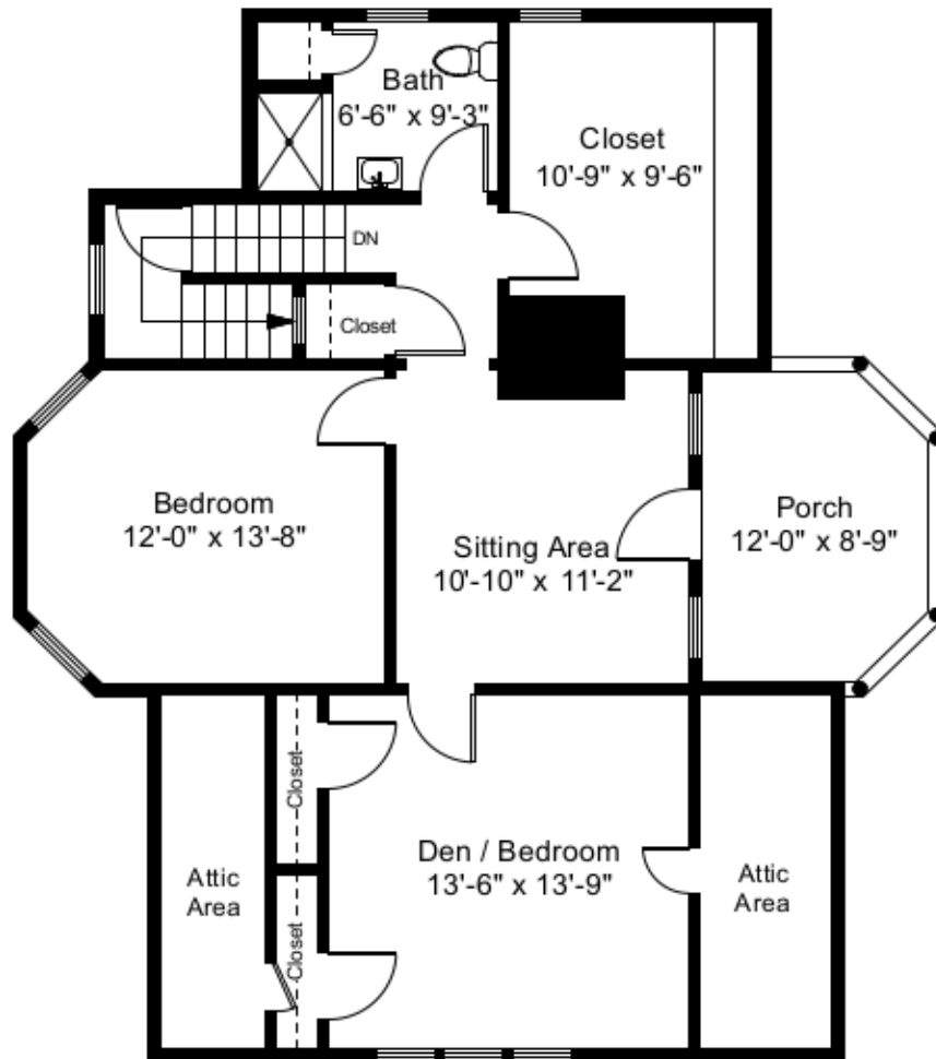
Third Floor Plan Ceiling Height = 8'-0"
