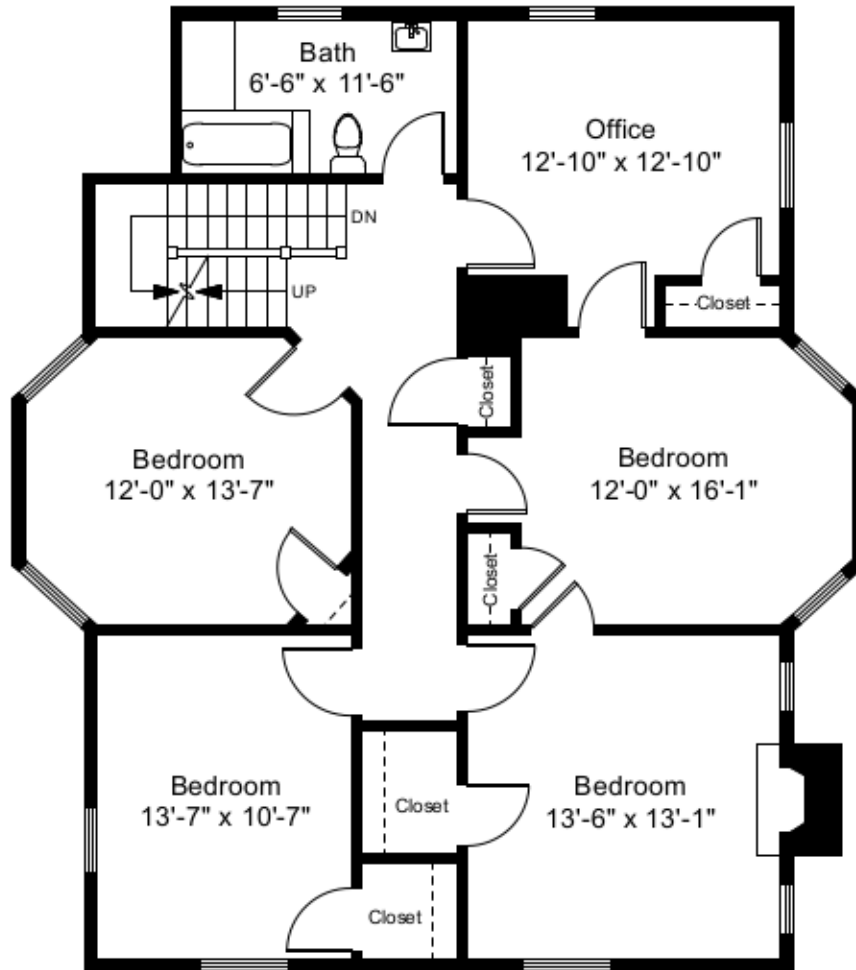
Second Floor Plan Ceiling Height = 8'-5"
