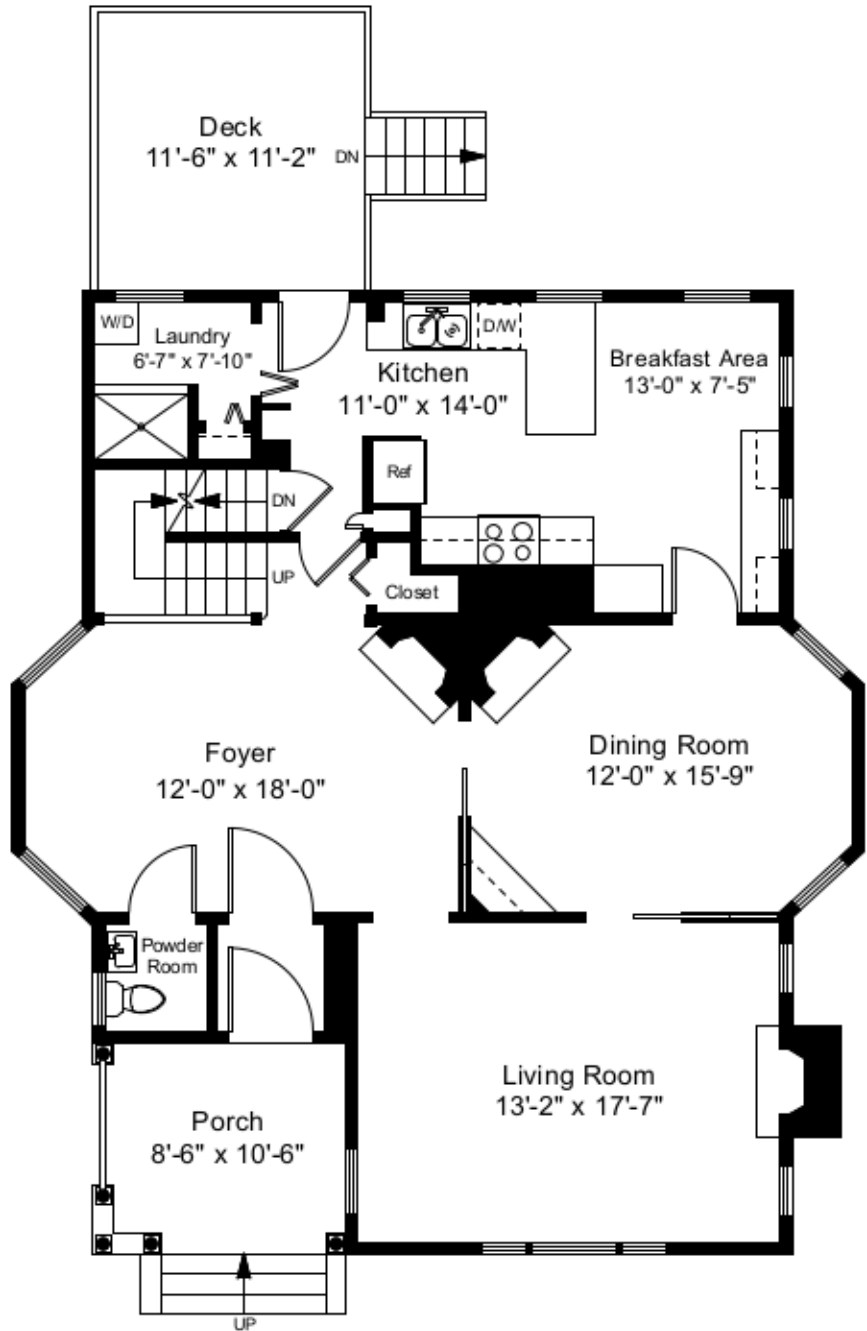
First Floor Plan Ceiling Height = 8'-10"
